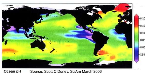
Fig. 5 Variations in pH in sea water
